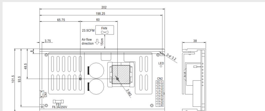
AC Input Connector (CN1) : JST B3P-VH or equivalent
